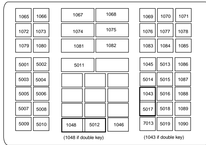
Figure 5-4. NCR 7052 58-KEY
