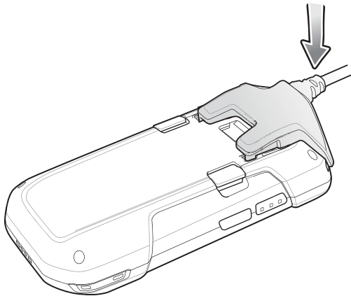
Figure 6-36 Press Down on Cable
