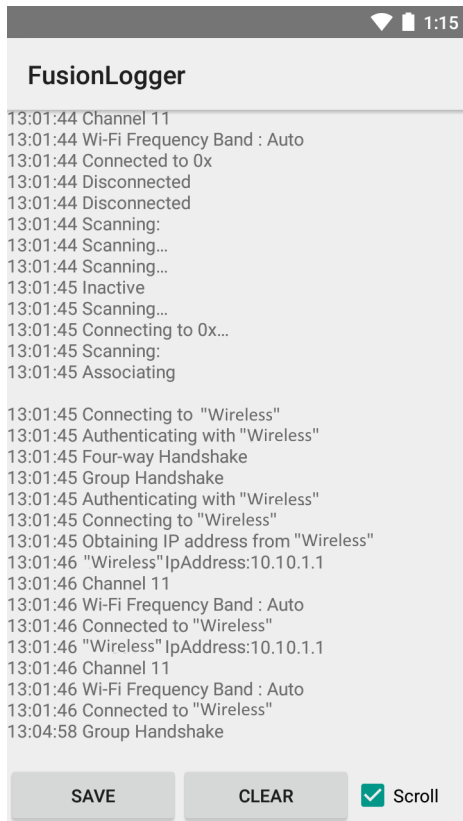
Figure 5-7 Fusion Logger Screen
