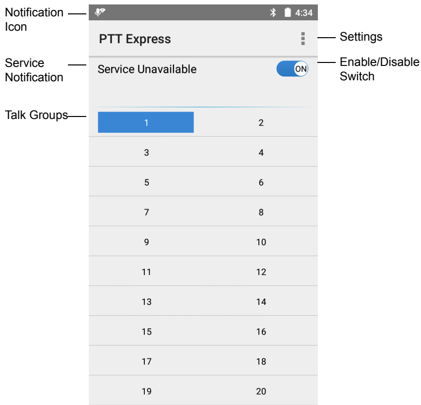
Figure 3-20 PTT Express Default User Interface (Enabled)
