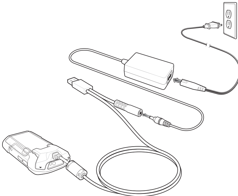
Figure 6-35 Power Setup
