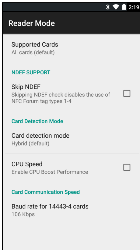
Figure 5-14 Reader Mode Settings
