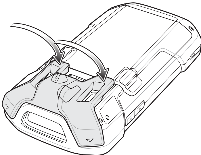
Figure 6-22 Rotate Audio Adapter onto TC70
