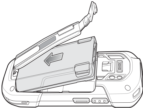
Figure 1-6 Insert Bottom of Battery into Battery Compartment
