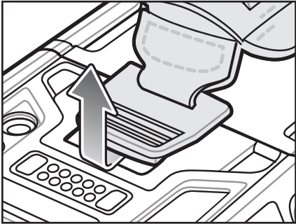
Figure 1-11 Remove Hand Strap Clip
