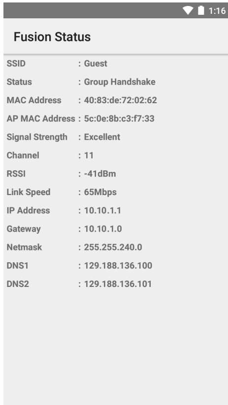
Figure 5-8 Fusion Status Screen
