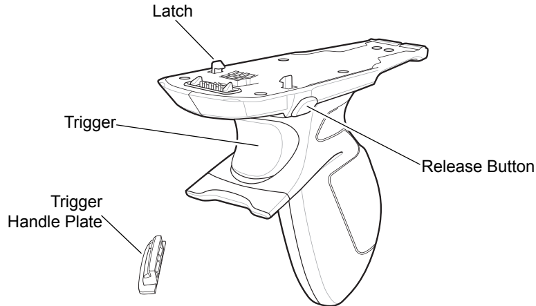
Figure 6-46 Trigger Handle
