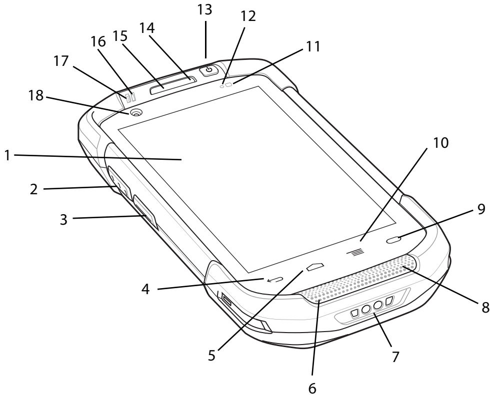
Figure 1-1 TC70 Front View
