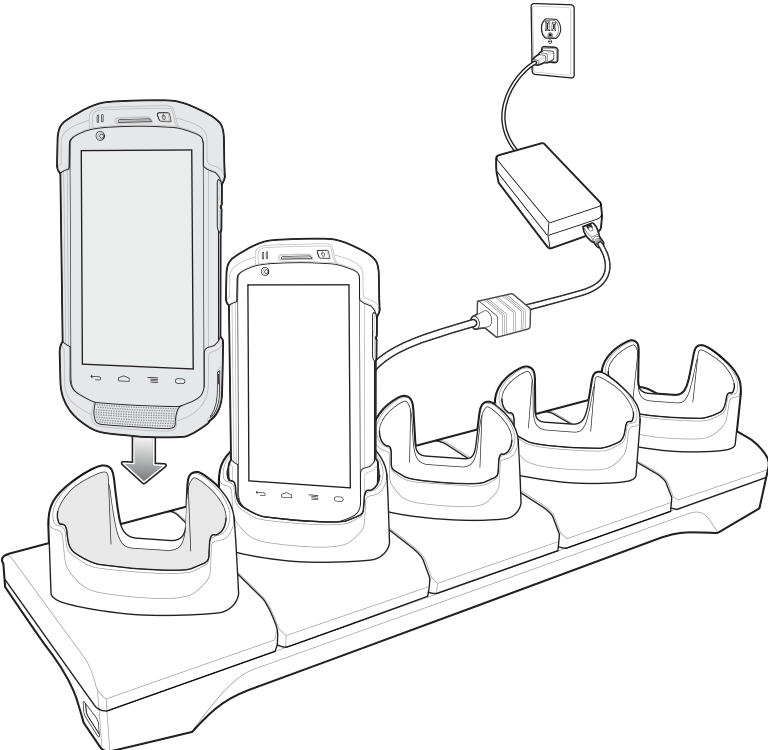
Figure 6-10 TC70 Battery Charging
