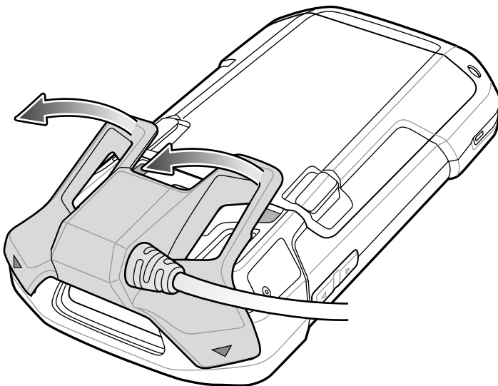
Figure 6-31 Remove Audio Adapter from TC70
