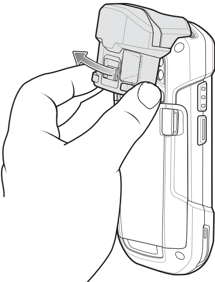
Figure 6-19 Remove MSR
