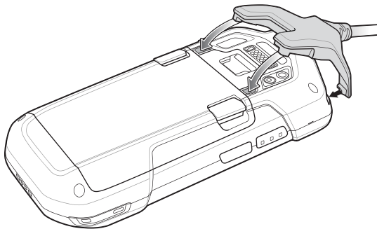
Figure 6-41 Cable Installation
