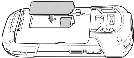
Figure 1-16 Replace Access Door
