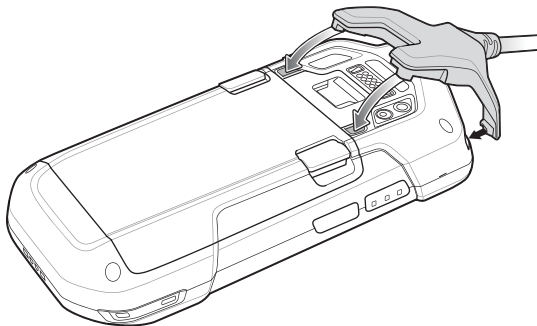
Figure 6-32 Cable Installation
