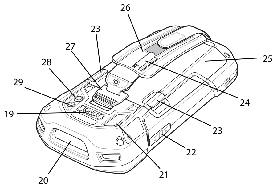
Figure 1-2 TC70 Rear View
