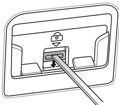
Figure 6-17 Lock MSR
